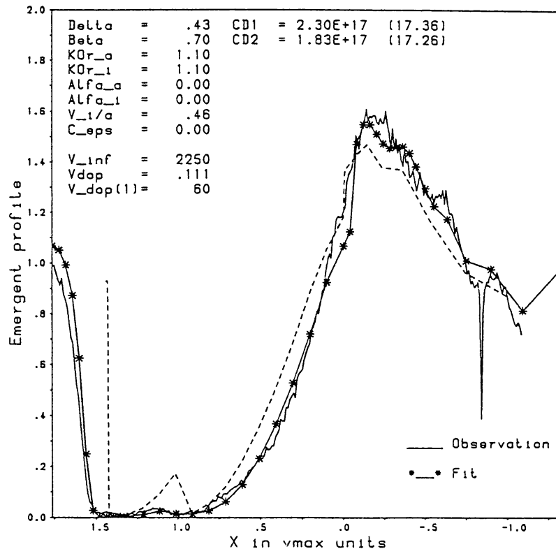
Figure 8: SEI-fit to the NV doublet of \zeta Pup using v_{turb}^{max} \approx 250 km/s . The dashed line shows the profile resulting from the same parameters, however with v_{turb} \equiv 0 . (From S. Haser, p.c.)
