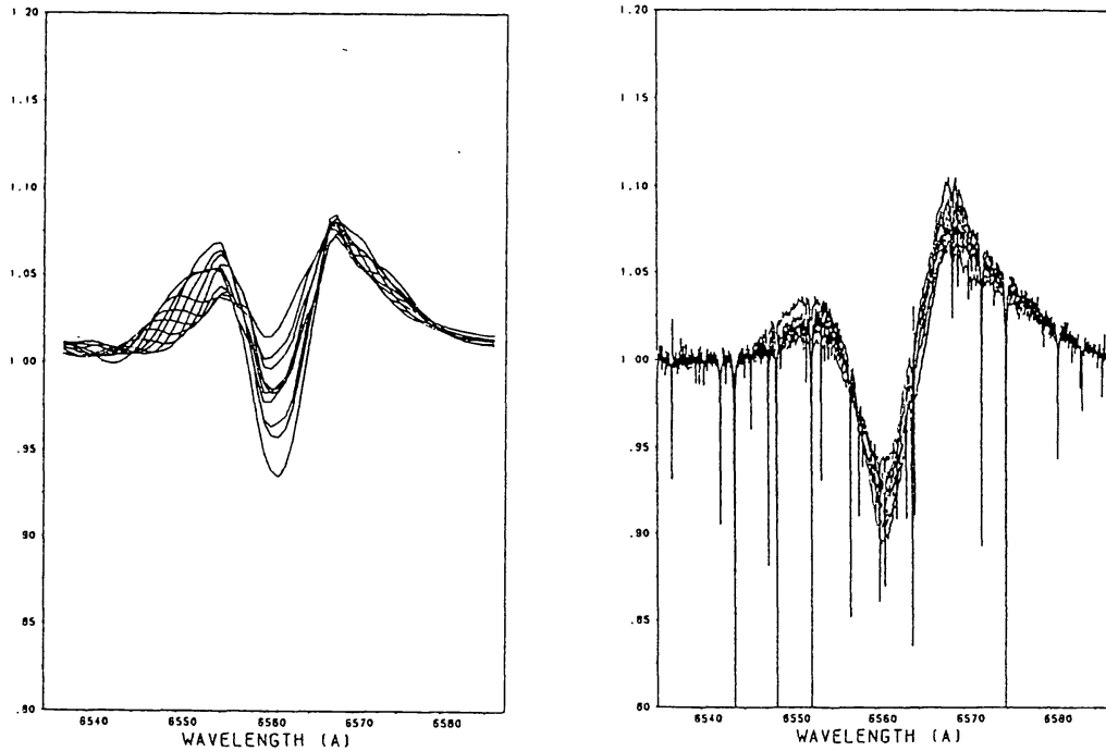
Figure 17: (a) Overlay of emergent H_\alpha -profiles for the structured wind at ten 1000-second intervals beginning at the snapshot Fig. 12. (b) Sequence of H_\alpha -observations of \zeta Pup (for details, see text, observations by D. Baade, p.c.).
