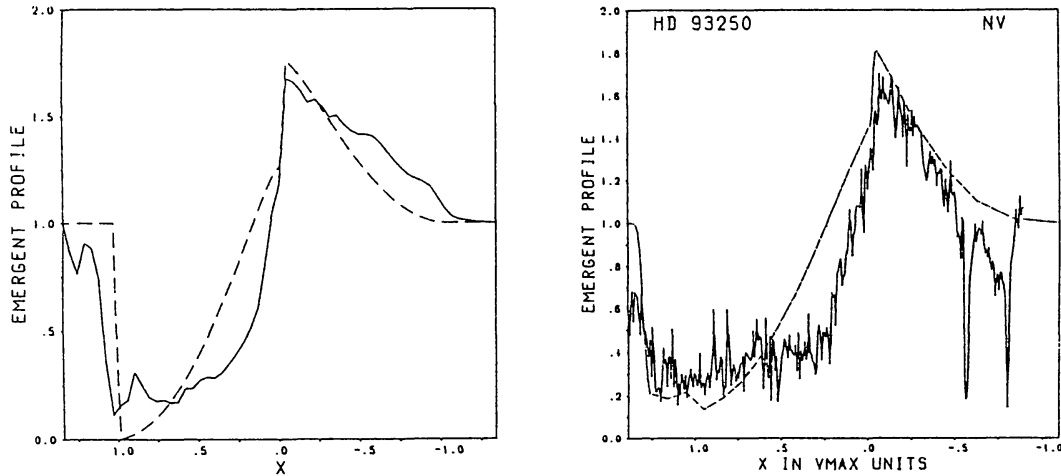
Figure 14: (left) Emergent profiles vs. dimensionless frequency x = (\nu/\nu_o - 1)c/v_{\text{mCAK}}(R_{\text{max}}) for a strong line and the structure-wind snapshot of Fig. 12 (fully drawn) and the smooth model (dashed). (From Puls and Owocki, 1993.)
